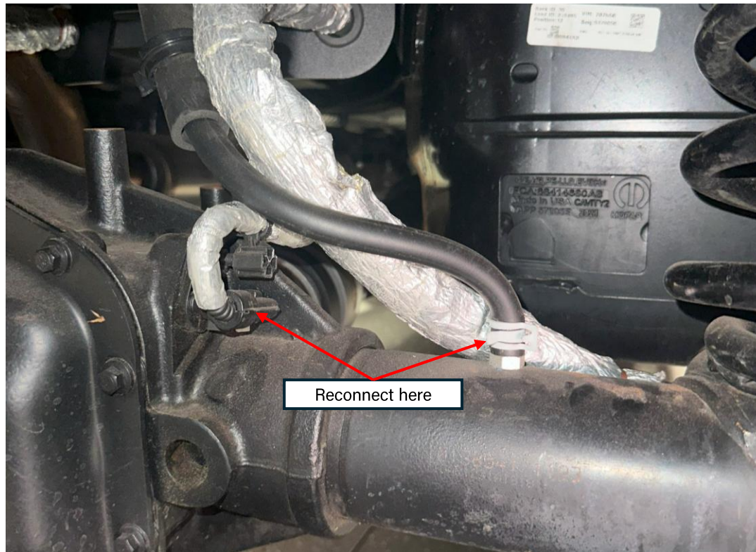
Figure 31: Differential wiring harness and breather tube reconnected
