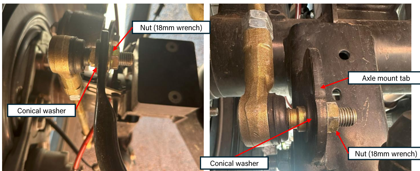
Figure 28: Sway bar end links installed on driver-side
